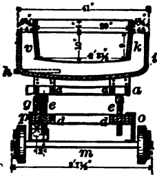
SECTION ON A B.
